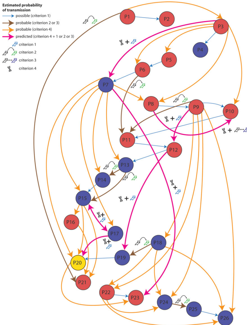
Figure 3. Estimated probability of transmission routes for 26 outbreak patients using the TPS algorithm. Each patient is outlined as a circle. The colour of the circle indicates the patient’s location at the first finding of the outbreak isolate. Red stands for ward 1, blue stands for ward 2 and yellow stands for the outpatient department. The line colour and thickness reflect the estimated strength of the transmission probability between two patients. Criteria 1–4 are described in detail in the Materials and methods section (as well as in the Supplementary data). Briefly: criterion 1, same ward, same time; criterion 2, same room consecutively within 14 days; criterion 3, same room, same time; and criterion 4, close genetic relatedness. The presence of criteria is indicated by symbols in close proximity to the line of transmission between two patients.
